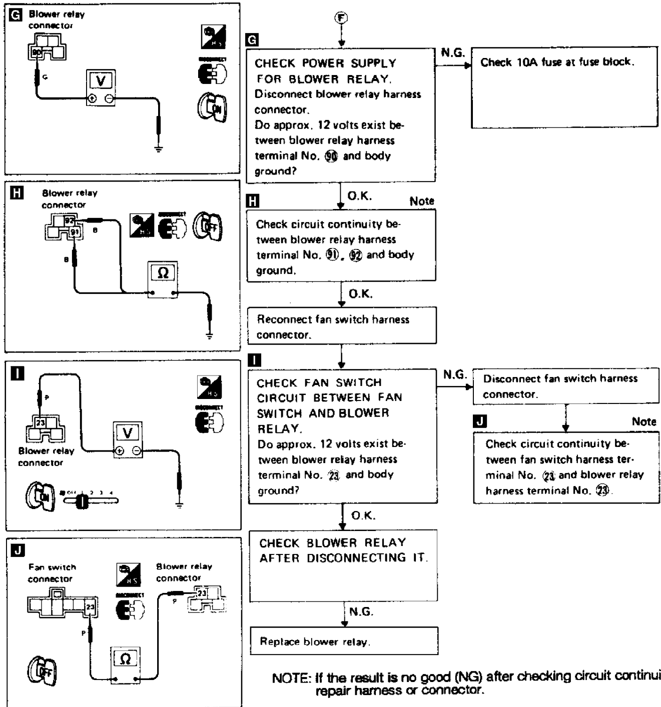
91D04815 Fig. 9: Diagnostic Procedure 1 (3 of 3) Courtesy of Nissan Motor Co., U.S.A.
