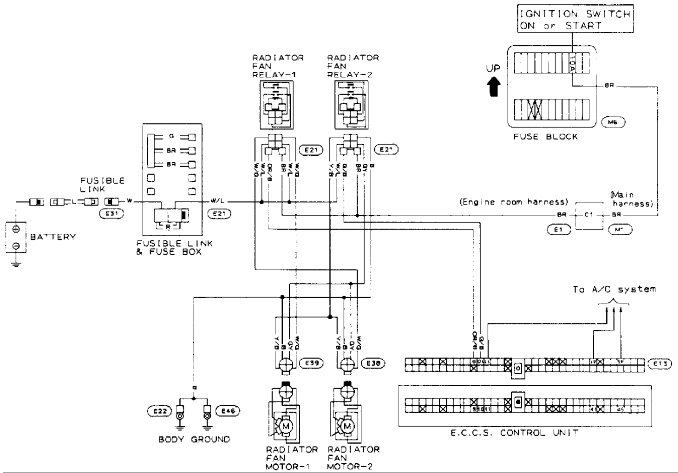
Fig. 2: Axxess Electric Cooling Fan Wiring Schematic
